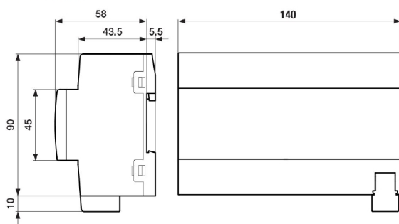
Dimension drawing
