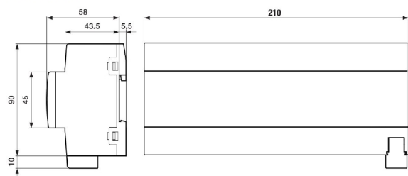
Dimension drawing
